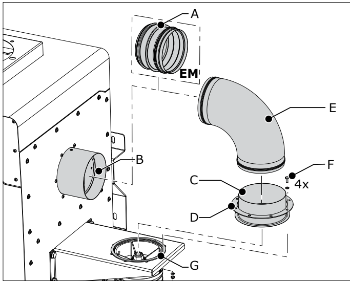
Fig. 4.13 Inlet ducting
