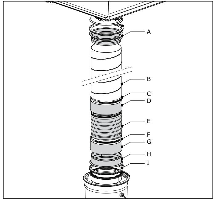
Fig. 4.15 Dustbin extension set
