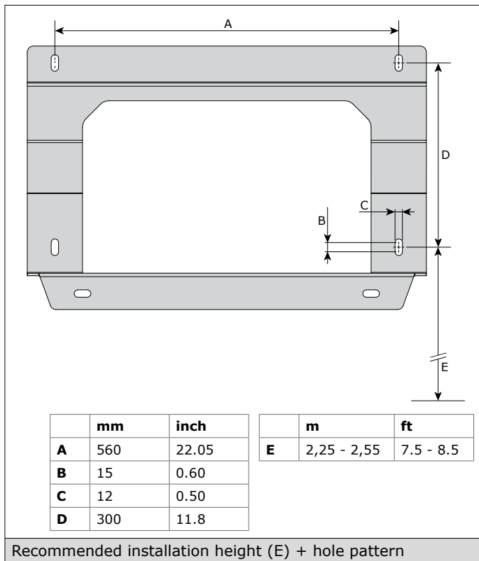
Fig. VI Installation height
