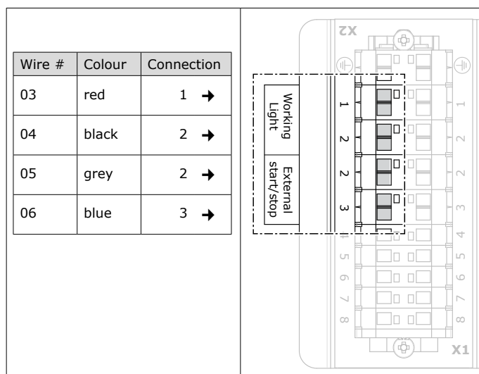
Fig. 4.12 Cable connection inside indicator panel
