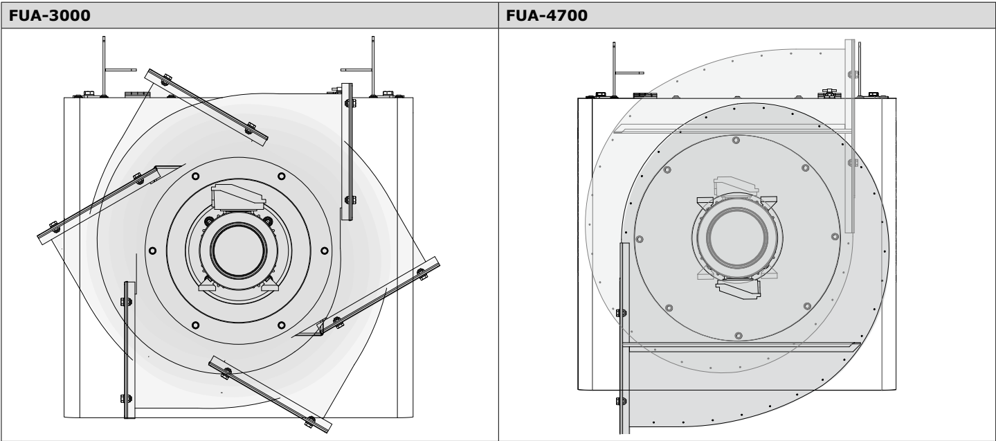
Fig. III Possible outlet directions of the fan
