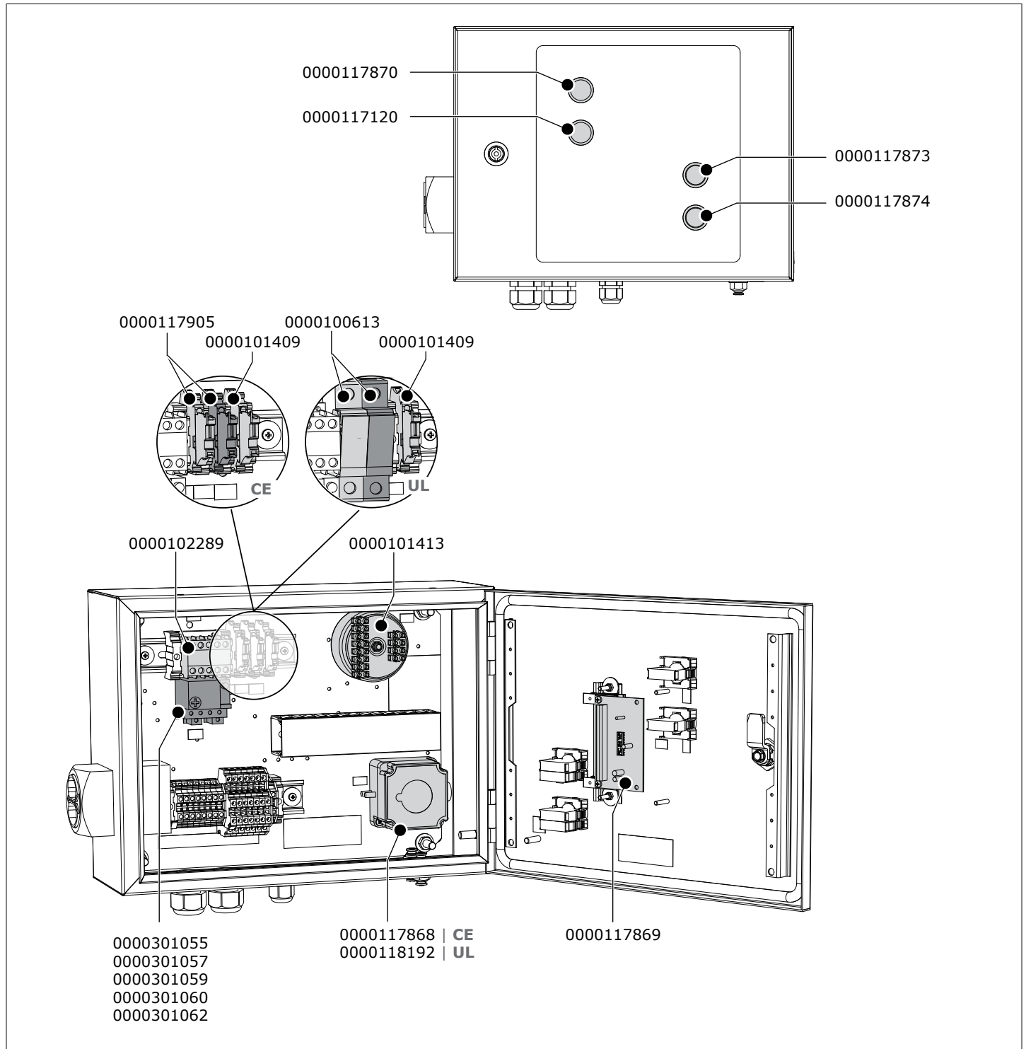
Fig. X Exploded view control box
