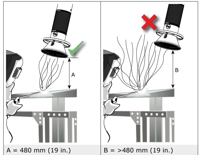
Fig. VII Positioning of the extraction arm
