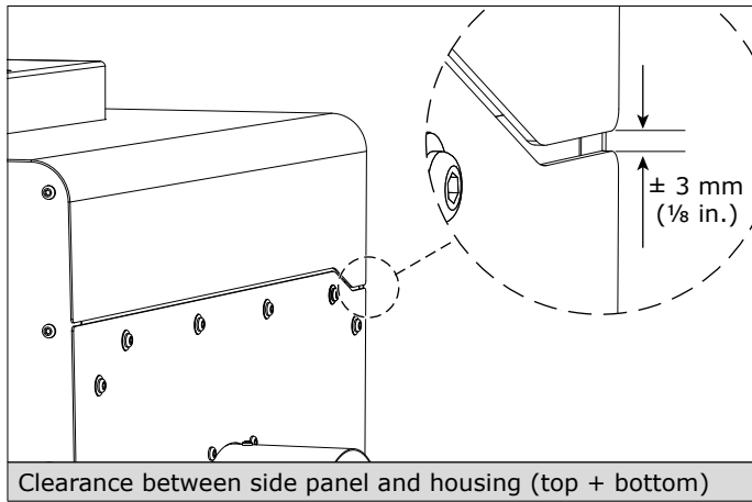
Fig. V Mounting position of the side panel
