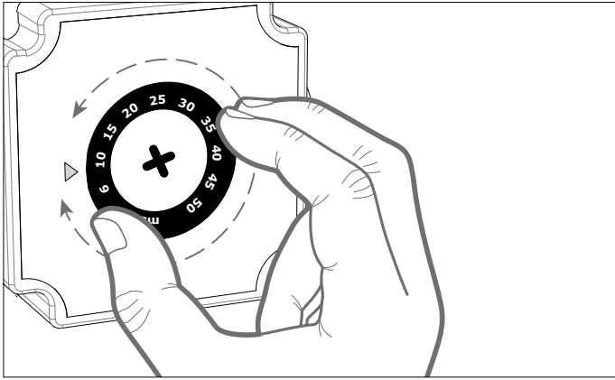
Fig. 4.18 Differential pressure switch
