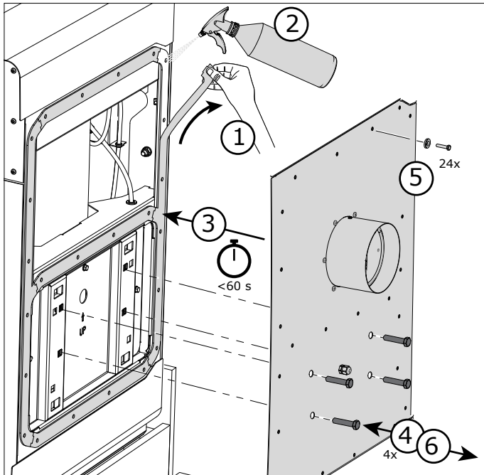
Fig. 4.4 Mounting of the side panel
