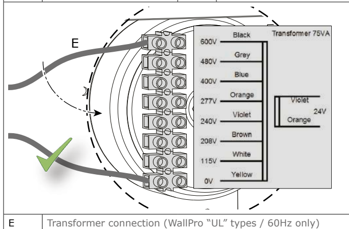
E Transformer connection (WallPro "UL" types / 60Hz only)
