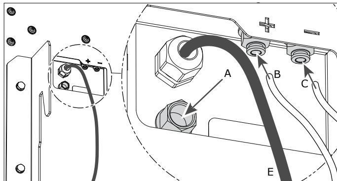
Fig. 4.8 Compressed air connection (rear of the unit)
