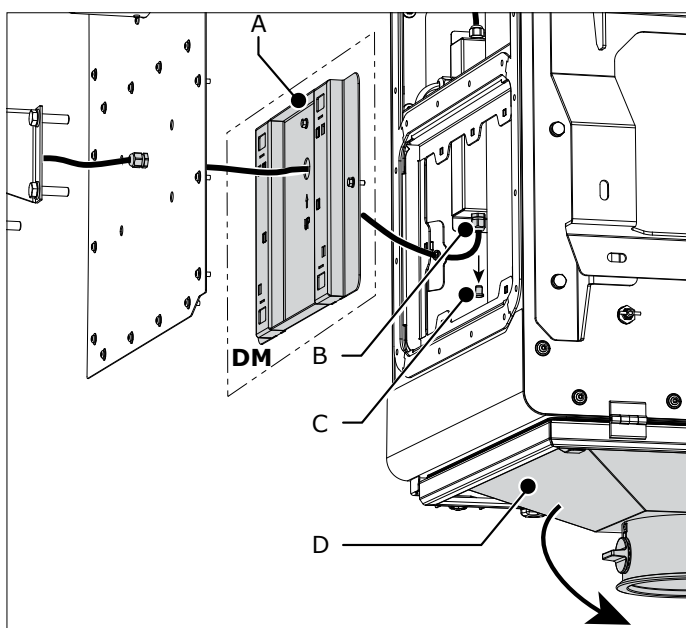
Fig. 4.11 Cable connection
