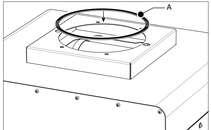
Fig. 4.6 Adhesive rubber strip
