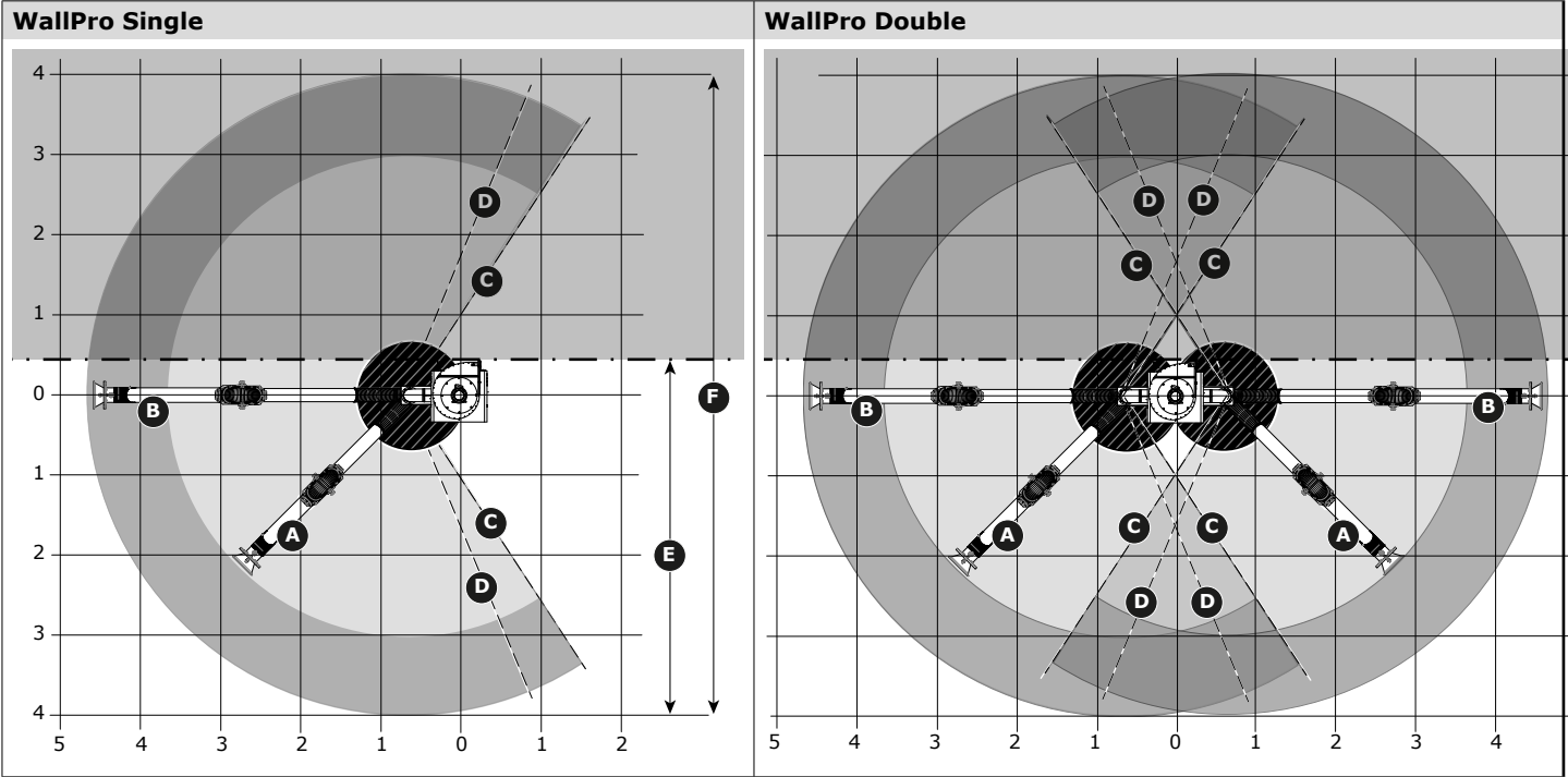
Fig. II Working range
