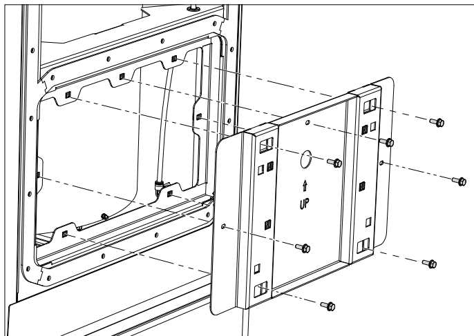
Fig. 4.2 Mounting of the reinforcement plate
