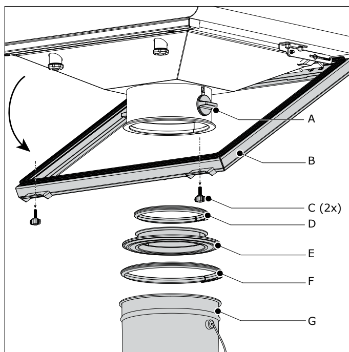
Fig. 6.1 Bag frame
