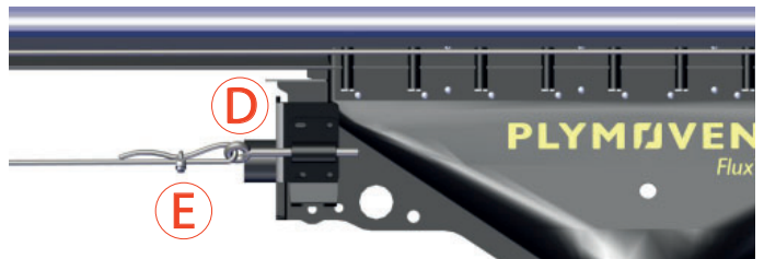
Fig. 4.3.11 Installing the rope
