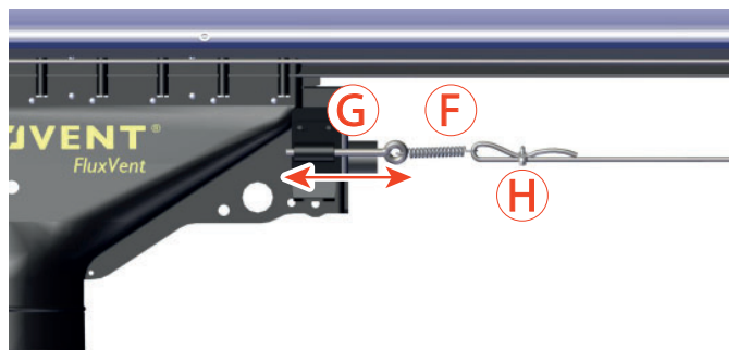
Fig. 6.3.11 Installing the rope
