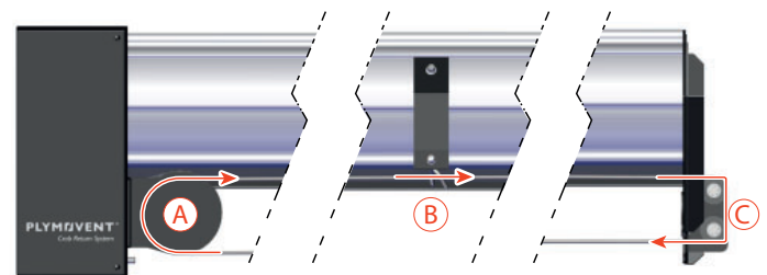
Fig. 5.3.9 Installing the rope
