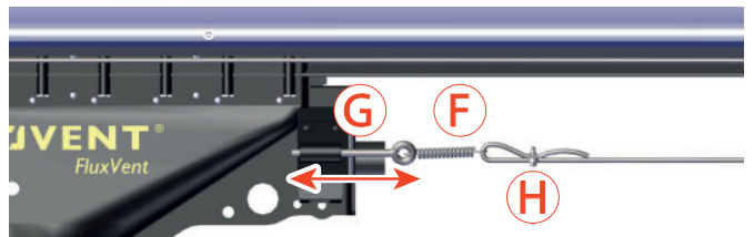
Fig. 4.3.12 Installing the rope
