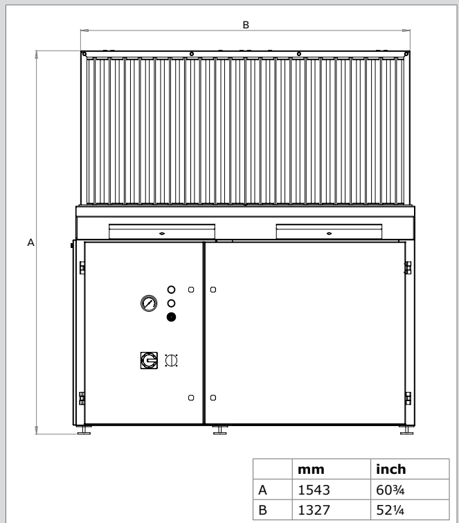
Downdraft table with backdraft kit (front view)
