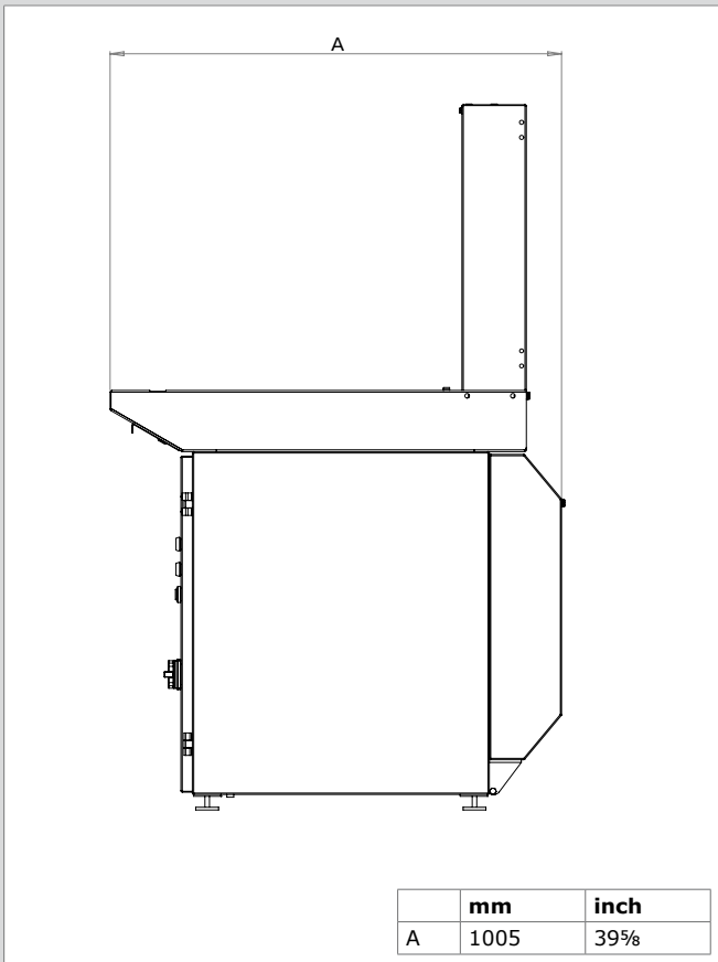
Downdraft table with backdraft kit (side view)
