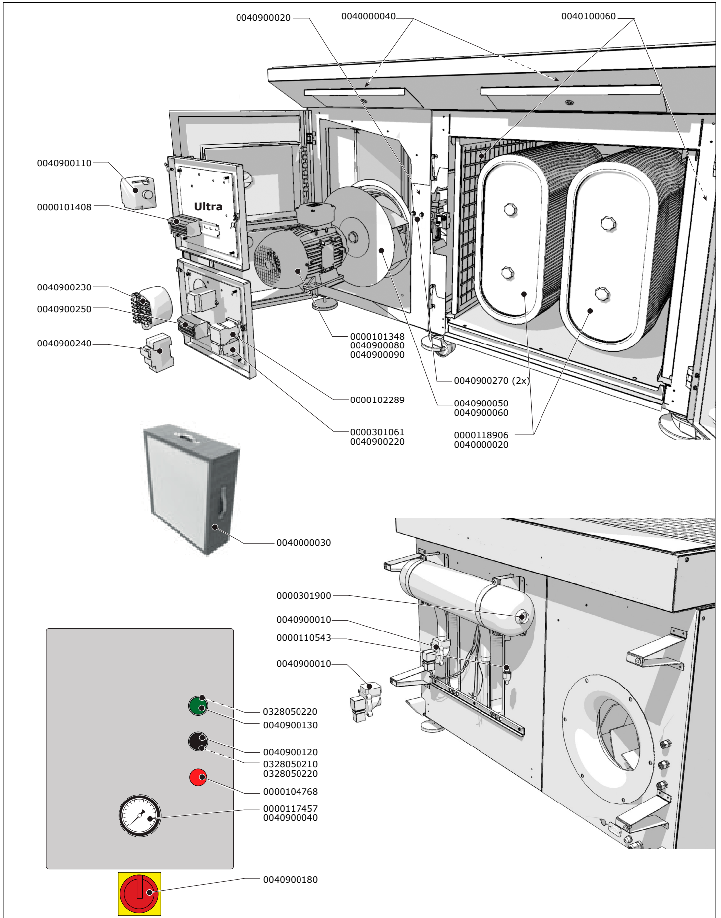
Fig. IV Exploded view
