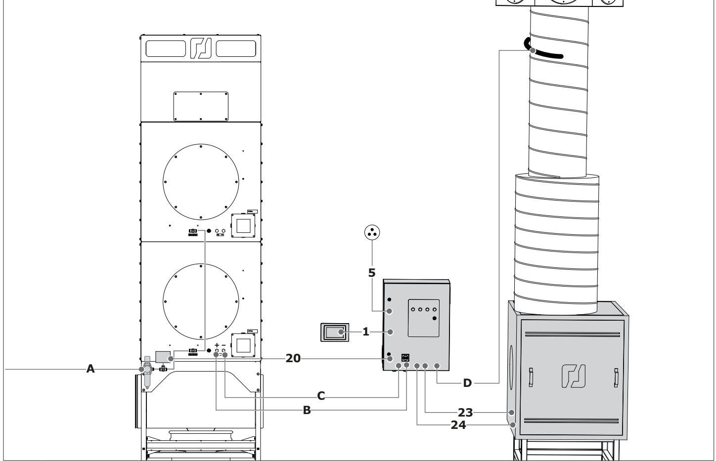
Fig. V Control panel
