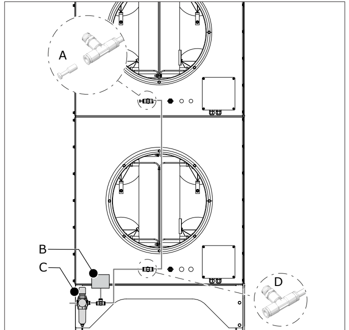
Fig. 4.23 Pressure hose
