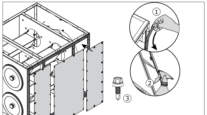
Fig. 4.24 Cover plates
