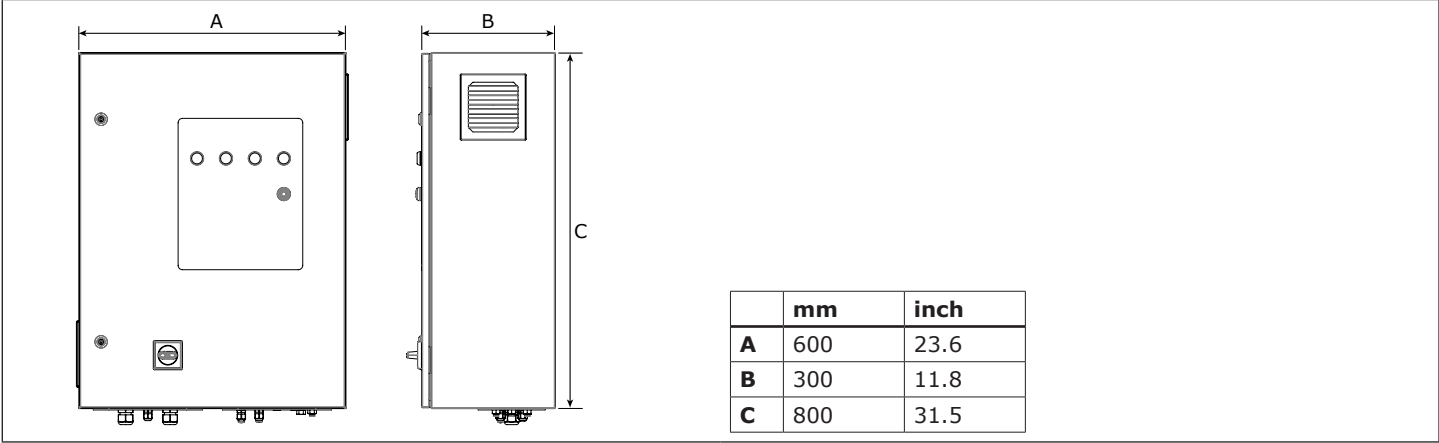
Fig. II Dimensions Panel
